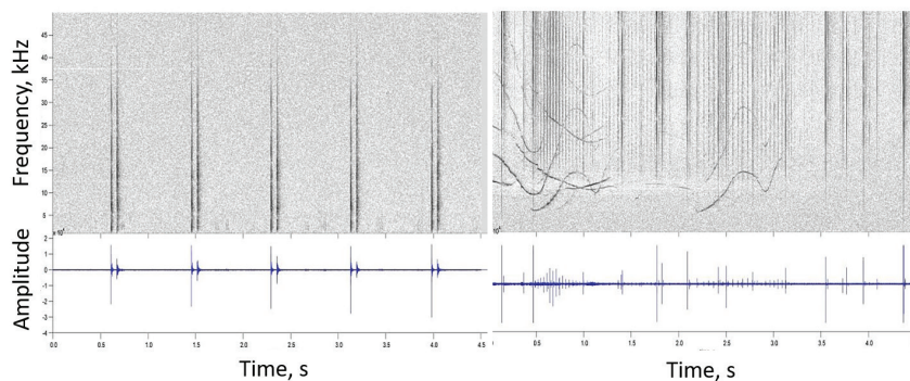
Fig. 2: Spectrogram (1024 Fast-Fourier Transform, Hamming window, 50% overlap) (top panels) and waveform (bottom panels) of sperm whale usual clicks (on the left; showing clicks and their surface reflection) and delphinid clicks and whistles (on the right) recorded by a Passive Aquatic Listener (PAL) (duration: 4.5 s, sampled at 100 kHz) at Pylos and Athos Stations, respectively.
